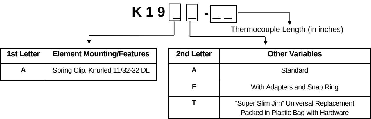
Figure 8: K19 Thermocouple
